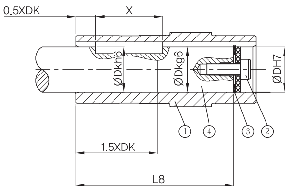
(A) User Shaft without Contact Shoulder
