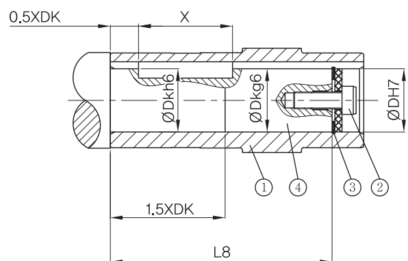
(B) User Shaft with Contact Shoulder
