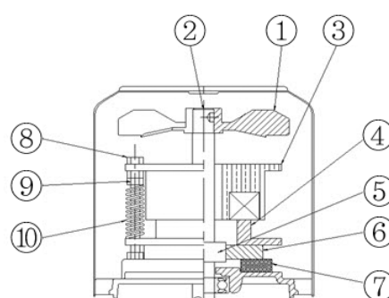
DC-B TYPE (HBV SERIES)
