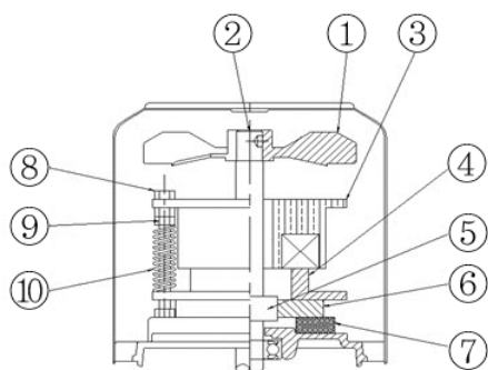
AC-B TYPE (SHB SERIES)
