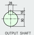
OUTPUT SHAFT
